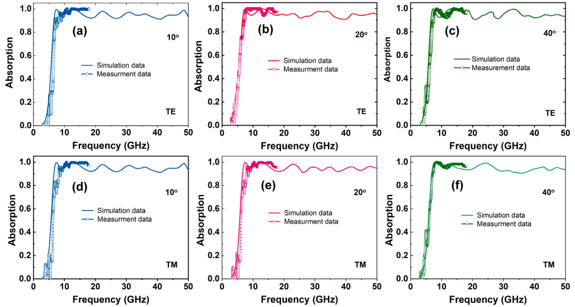
Fig. 11. The simulated and measured results of absorption spectra of the proposed UWBWMA under different incident angles of (a), (d) 10^\circ , (b), (e) 20^\circ , and (c), (f) 40^\circ for TE and TM modes, respectively.
