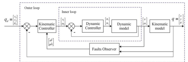
Figure 2. Structure of FTC
