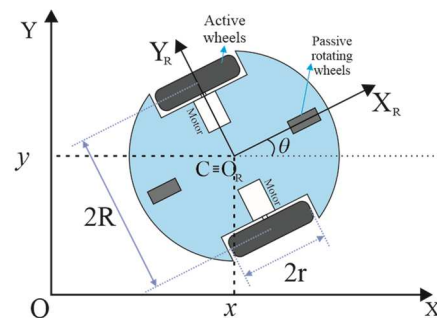
Figure 1. Differential-drive mobile robot
