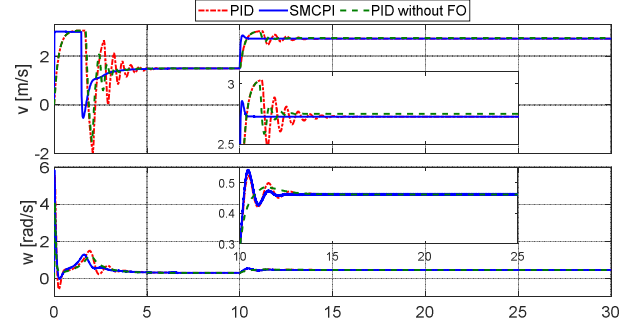
Figure 5. Linear and Angular velocities.
