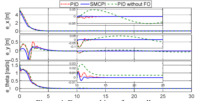
Figure 4. Error tracking of controllers.
