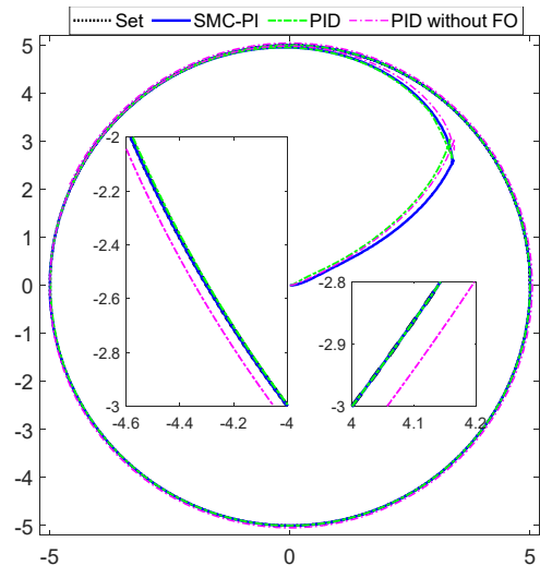
Figure 7. Tracking follows the set trajectory
