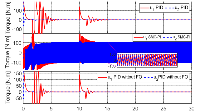
Figure 6. Controller's signal.
