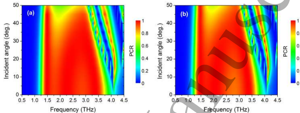
Figure 7. The PCR map of the proposed polarization converter as a function of the frequency and the incident angle for (a) TE and (b) TM polarizations.
