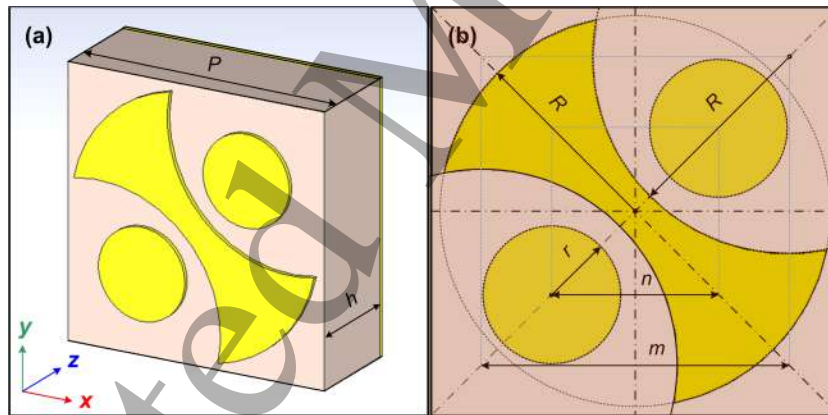
Figure 1. Geometry of the proposed converter: (a) perspective and (b) top views.
