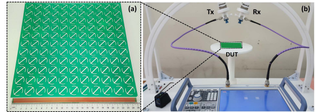
FIGURE 8. (a) Photo of fabricated polarization converter which consists of 11 \times 11 unit cells, and (b) Measurement setup for the fabricated prototype.
