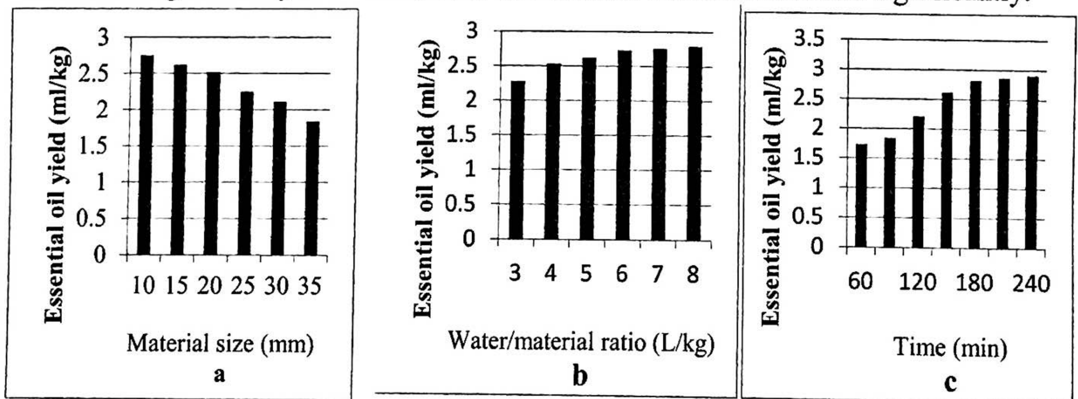
Figure 1: The effect of material size (a), water/material ratio(b), distillation time (c) on essential oil yield
