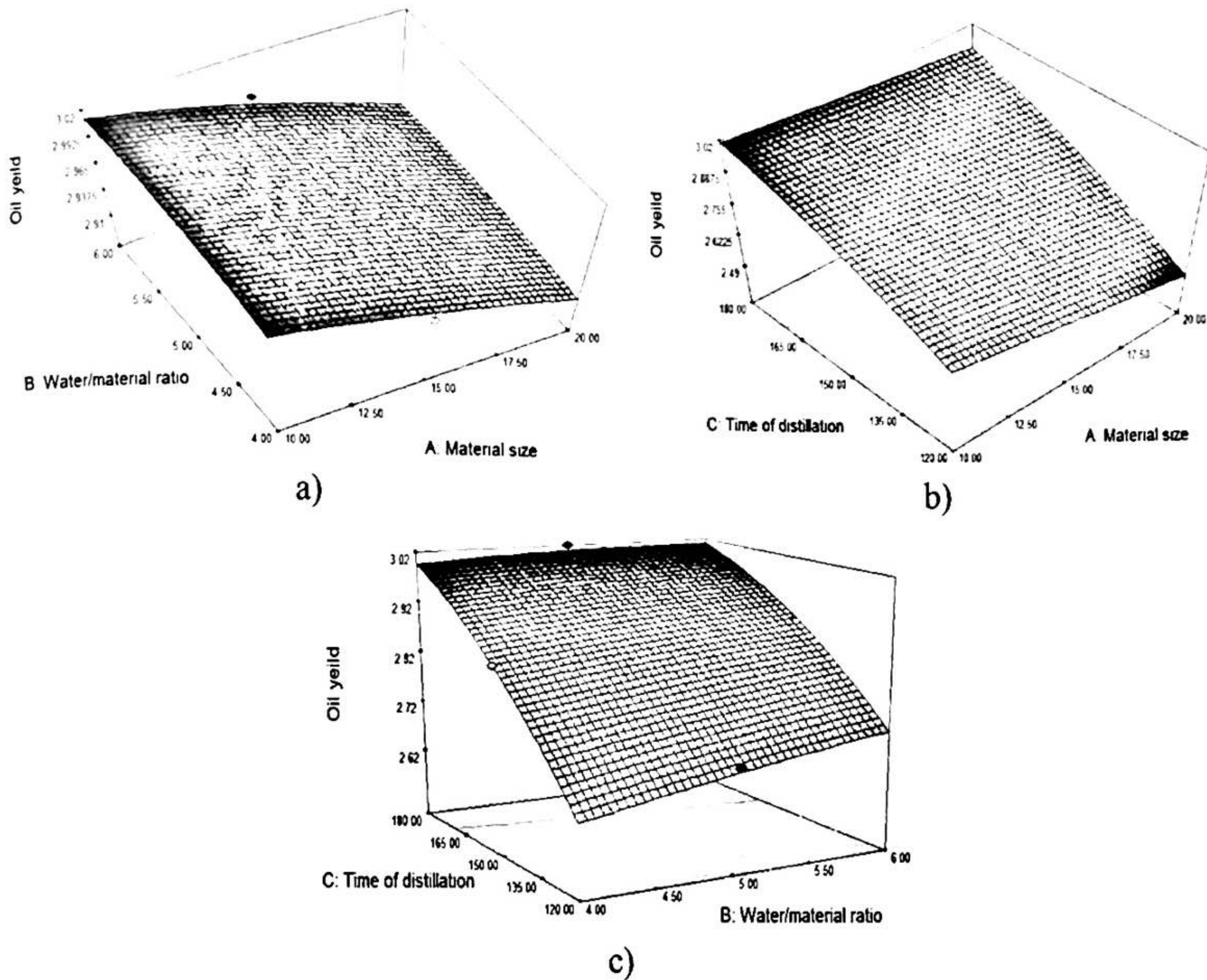
Figure 2: Response surface of oil yield
