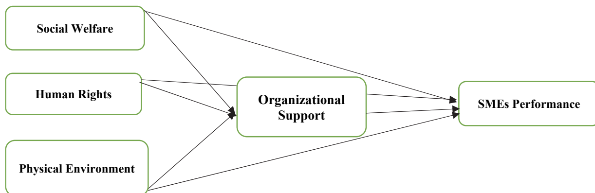
Fig. 2. Theoretical Model
