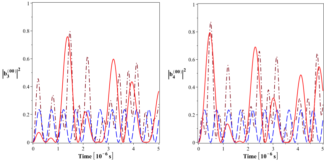
Figure 2: The probabilities to the system exist in the Bell-like states |B_3^{(00)}\rangle and |B_4^{(00)}\rangle for the coupler pumped in one mode with \alpha = \varepsilon = 10^6 \pi \text{ rad/s} , \beta = 0 (solid line) and in two modes with \alpha = \varepsilon = \beta = 10^6 \pi \text{ rad/s} (dashed line) and \alpha = \varepsilon = \beta/2 = 10^6 \pi \text{ rad/s} (dashed dotted line).
