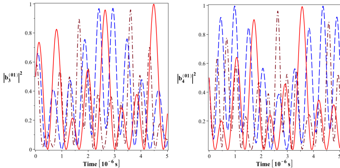
Figure 3: The probabilities to the system exist in the Bell-like states |B_3^{(01)}\rangle and |B_4^{(01)}\rangle for the coupler pumped in one mode with \alpha = \varepsilon = 10^6 \pi \text{ rad/s} , \beta = 0 (solid line) and in two modes with \alpha = \varepsilon = \beta = 10^6 \pi \text{ rad/s} (dashed line) and \alpha = \varepsilon = \beta/2 = 10^6 \pi \text{ rad/s} (dashed dotted line).
