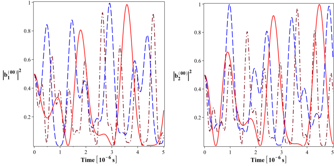
Figure 1: The probabilities to the system exist in the Bell-like states |B_1^{(00)}\rangle and |B_2^{(00)}\rangle for the coupler pumped in one mode with \alpha = \varepsilon = 10^6 \pi \text{ rad/s} , \beta = 0 (solid line) and in two modes with \alpha = \varepsilon = \beta = 10^6 \pi \text{ rad/s} (dashed line) and \alpha = \varepsilon = \beta/2 = 10^6 \pi \text{ rad/s} (dashed dotted line).
