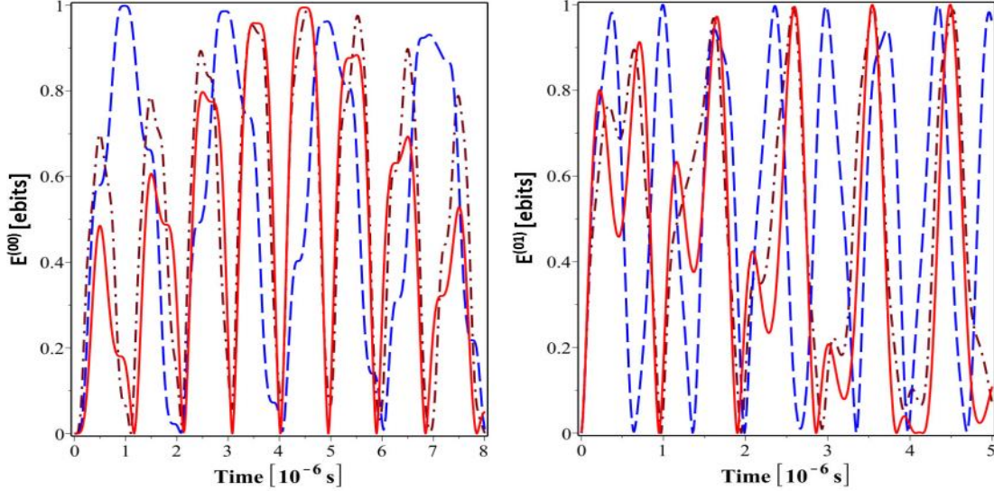
Figure 4: Evolution of the entropies of entanglement E^{(00)} and E^{(01)} for the coupler pumped in one mode with \alpha = \varepsilon = 10^6 \pi rad/s, \beta = 0 (solid line) and in two modes with \alpha = \varepsilon = \beta = 10^6 \pi rad/s (dashed line) and \alpha = \varepsilon = \beta/2 = 10^6 \pi rad/s (dashed dotted line).
