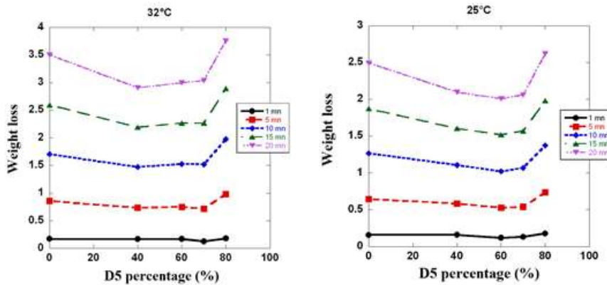
Fig-2: Loss weight versus the percentage of coarse sand
