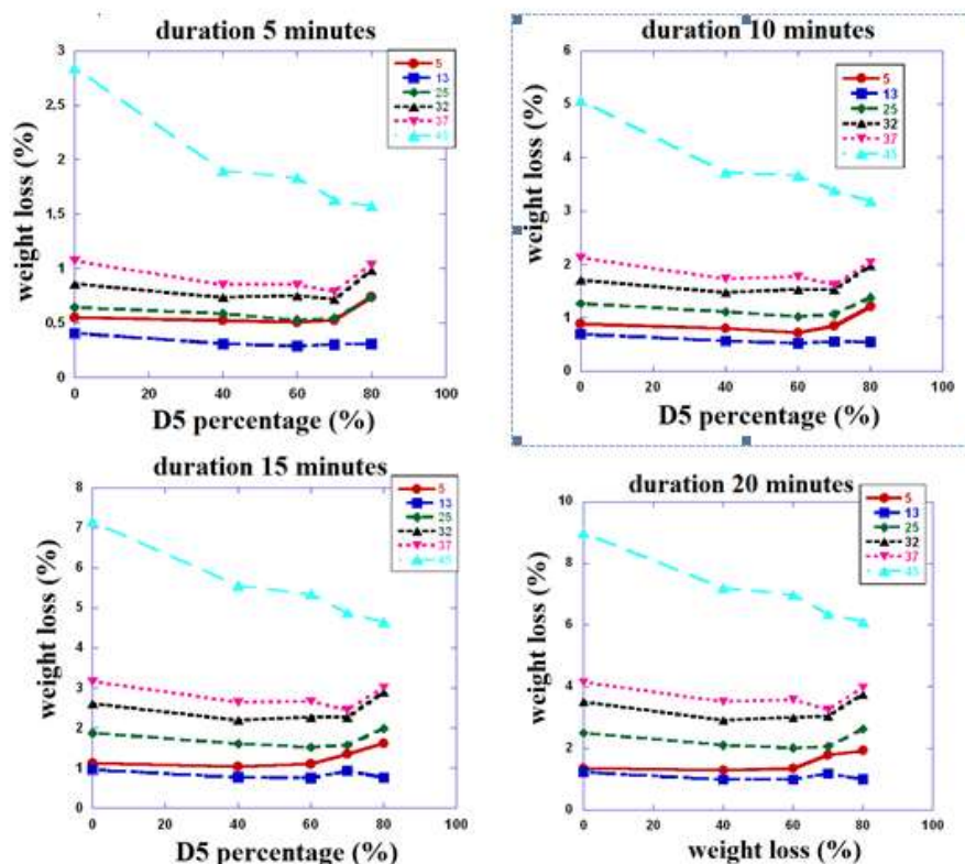
Fig-3: Comparison of the weight loss versus the percentage of coarse sand D5 at various relaxation time
